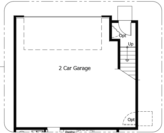
OPTIONAL GARAGE STAIRS w/ REAR DOOR (TO OPTIONAL STORAGE / OPTIONAL MULTI-GEN SUITE ABOVE)
