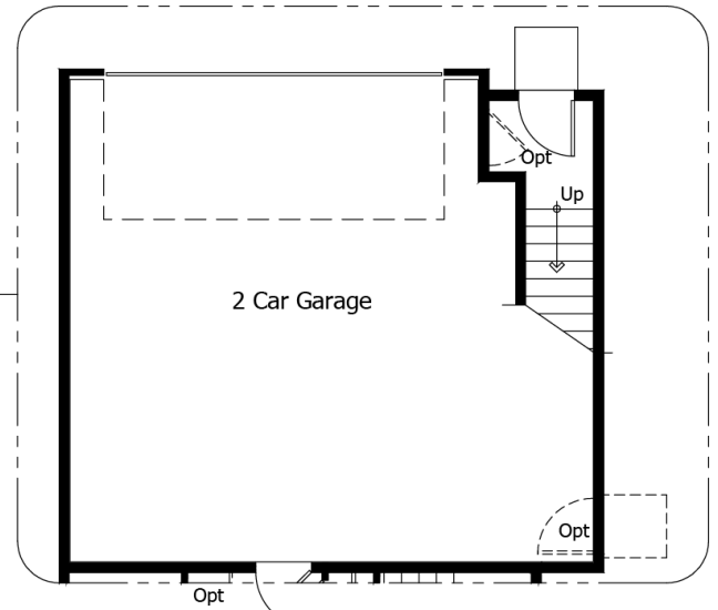
OPTIONAL GARAGE STAIRS & REAR DOOR (TO OPTIONAL STORAGE / OPTIONAL MULTI-GEN SUITE ABOVE)
