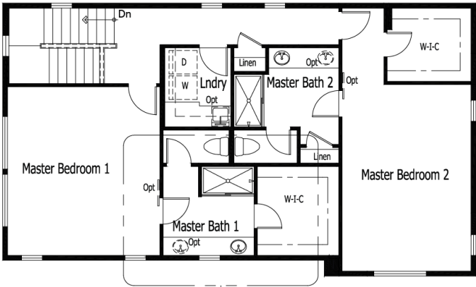
Optional Double Master Bedroom Layout
