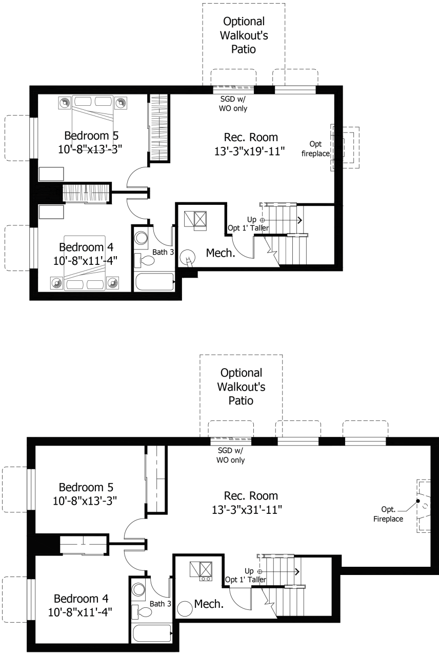
Basement Level w/ Opt. Finish (Shown w/ Opt. 3-car Garage with Study Included Above)
