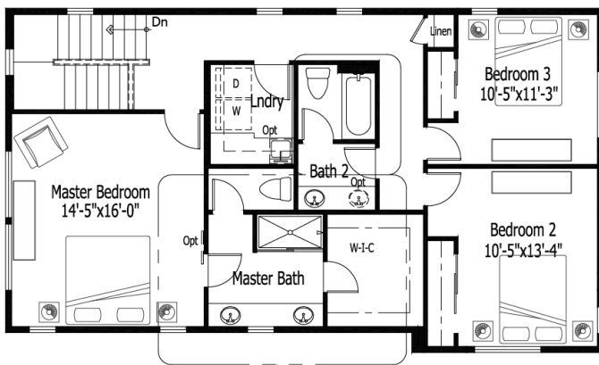
Standard 3 Bedroom Layout
